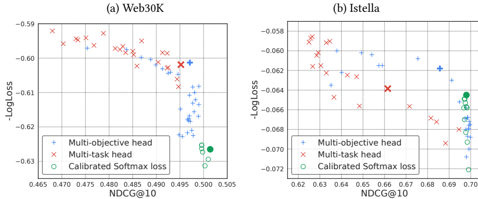
Figure 2: Tradeoffs of methods for logistic ranking and calibration. Negative LogLoss (-LogLoss) is used for illustration.
