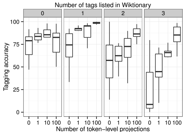
Figure 4: Relative influence of token and type constraints on tagging accuracy in the \hat{Y}^{\text{CRF}}_{\text{wik}}_{\text{C+L}} model. Word types are categorized according to a) their number of Wiktionary tags (0,1,2 or 3+ tags, with 0 representing no Wiktionary entry; top-axis) and b) the number of times they are token-constrained in the training set (divided into buckets of 0, 1-9, 10-99 and 100+ occurrences; x-axis). The boxes summarize the accuracy distributions across languages for each word type category as defined by a) and b). The horizontal line in each box marks the median accuracy, the top and bottom mark the first and third quartile, respectively, while the whiskers mark the minimum and maximum values of the accuracy distribution.
