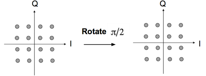
Fig. 9. Schematic illustration of cyclic phase slipping problem
