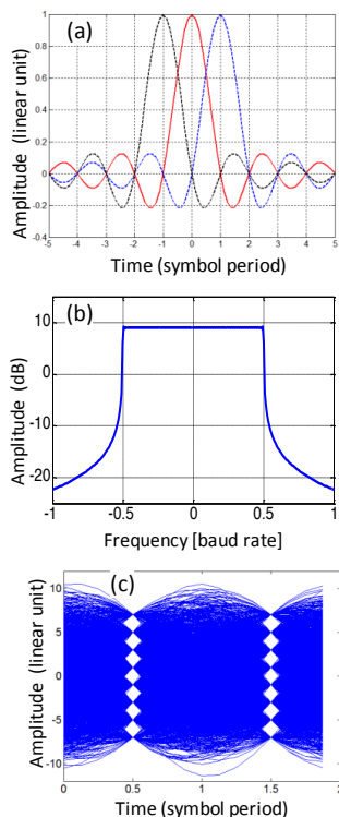
Fig. 6. Simulations of Nyquist pulse signaling: (a) illustration of three Nyquist pulses in the time domain; (b) frequency-domain spectrum with roll-off factor=0.01 and (c) eye diagram of a Nyquist-shaped 32-64 hybrid QAM signal.
