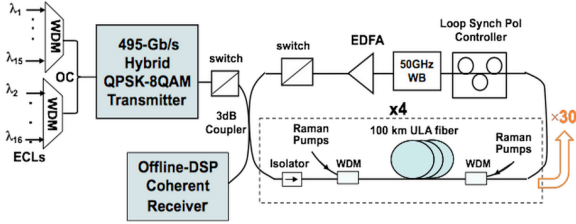
Fig. 19. 100GHz-spaced-8x495Gbit/s DWDM transmission setup.
