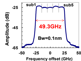
Fig. 7. Optical spectrum of a 495Gb/s PDM hybrid 32-64QAM signals generated using five subcarriers.
