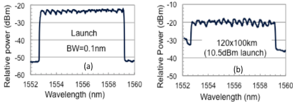
Fig. 20. Optical spectra measured prior to and after 12000km transmission.
