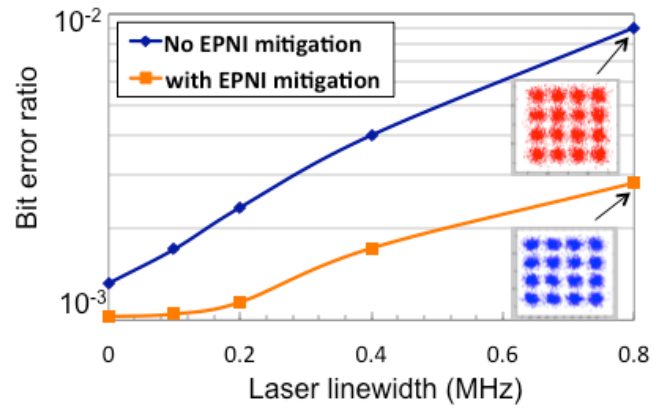
Fig. 14. Simulated BER performance vs. laser linewidth for a 7channel 49Gbaud PDM-16QAM WDM system (at 3dBm launch power and 2000km transmission of an ultra-large area fiber) with and without using the proposed EPNI mitigation technology.
