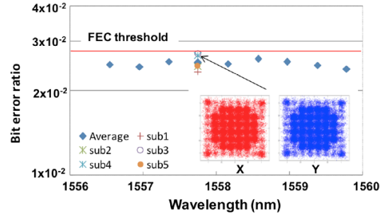
Fig. 18. Measured BER of ten 494.85Gb/s DWDM channels after 3200km transmission.
