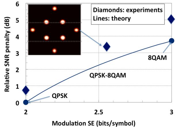
Fig. 4. Back-to-back SNR penalties for QPSK, hybrid QPSK-8QAM, and 8QAM, all operating at 9.7Gbaud and relative to theoretical QPSK sensitivity.
