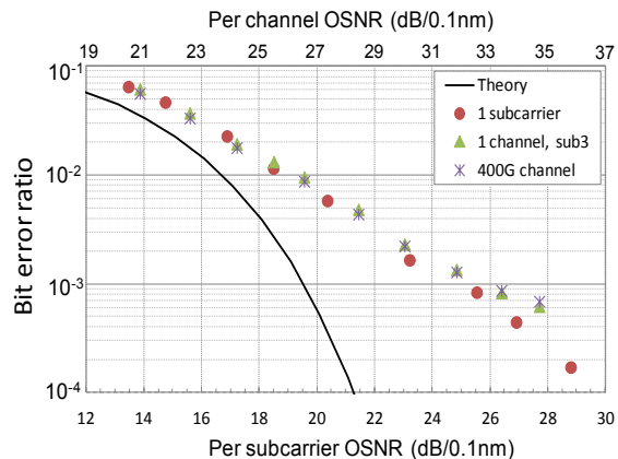
Fig. 8. Measured back-to-back BER performance versus OSNR under three different conditions for a 495Gb/s PDM hybrid 32-64QAM signal consisting of five subcarriers.
