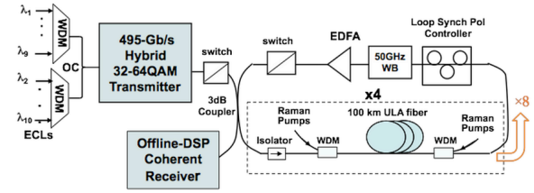
Fig. 16. 50GHz-spaced, 10×494.85Gbit/s DWDM transmission setup,
