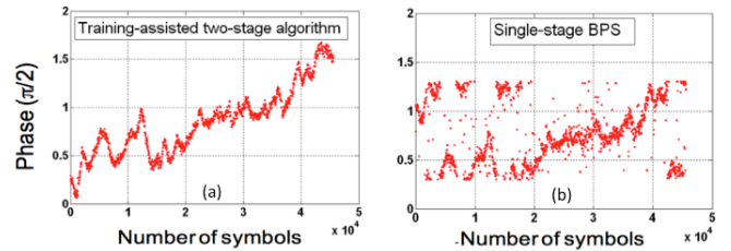
Fig. 11. Recovered carrier phases using two different algorithms: training-assisted two-stage algorithm and single-stage blind phase search algorithm, for a 400G WDM transmission experiment using a time-domain hybrid PDM-32-64QAM modulation format.
