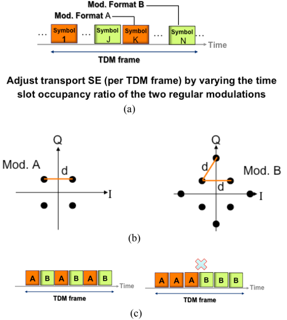
Fig. 2. Schematic illustration of the proposed time-domain hybrid QAM technique. (a) Concept of time-domain hybrid QAM; (b) equal Euclidean distance design concept for optimal linear performance and (c) uniform symbol distribution design concept for optimal nonlinear performance.
