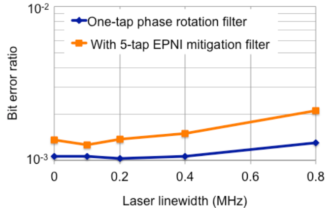
Fig. 15. Back-to-back performance comparison (OSNR=23dB) when using the conventional one-tap filter-based phase recovery method and the proposed multi-tap filter-based impairment mitigation method.
