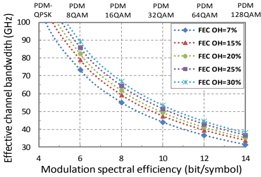
Fig. 1. Effective channel bandwidth versus modulation SE at several FEC code rates for a 400GigE system [9].
