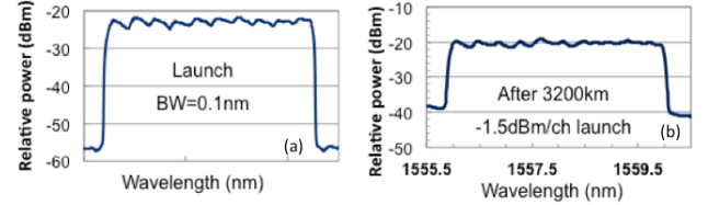
Fig. 17. Optical spectra measured prior to and after 3200km transmission.
