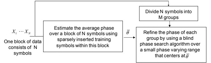
Fig. 10. Functional block illustration for the proposed phase recovery algorithm
