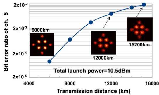
Fig. 21. Measured BER of the middle channel vs. transmission reach.
