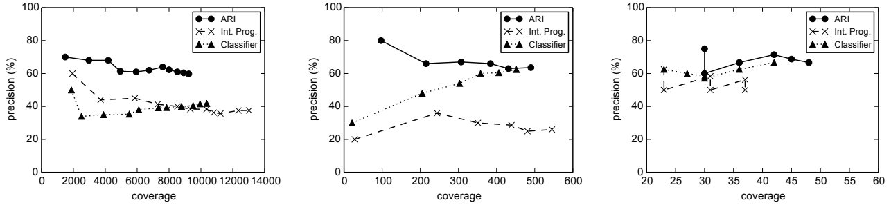
Figure 6: Rule Precision versus Coverage of top-500 rules of COUNTRIES (left), top-250 rules of US_PRESIDENTS (middle), and top-18 rules for DBpedia (right).
