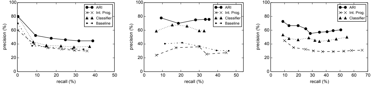
Figure 7: Attribute Precision versus Recall of 4135 attributes of COUNTRIES (left), 238 attributes of US_PRESIDENTS (middle), and 91 attributes of DBpedia (right).
