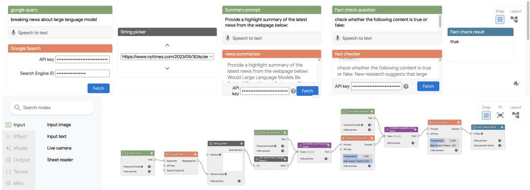
(a) Search news from Google, summarize it and then conduct fact check. Input: a keyword for Google Search; Output: a summarization of the news and a fact-check result.
