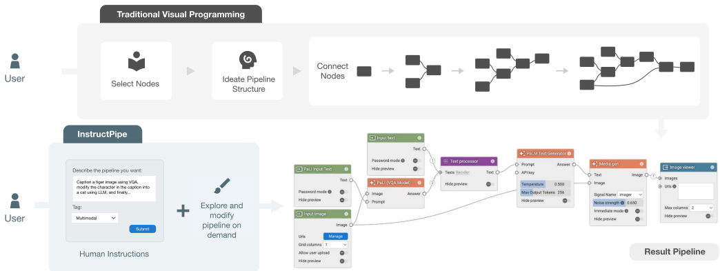
Fig. 1. Existing visual programming requires users to select nodes, conceive pipeline structure, and then create the pipeline starting from an empty workspace. In contrast, InstructPipe facilitates users to build interactive pipelines directly from text instructions.
