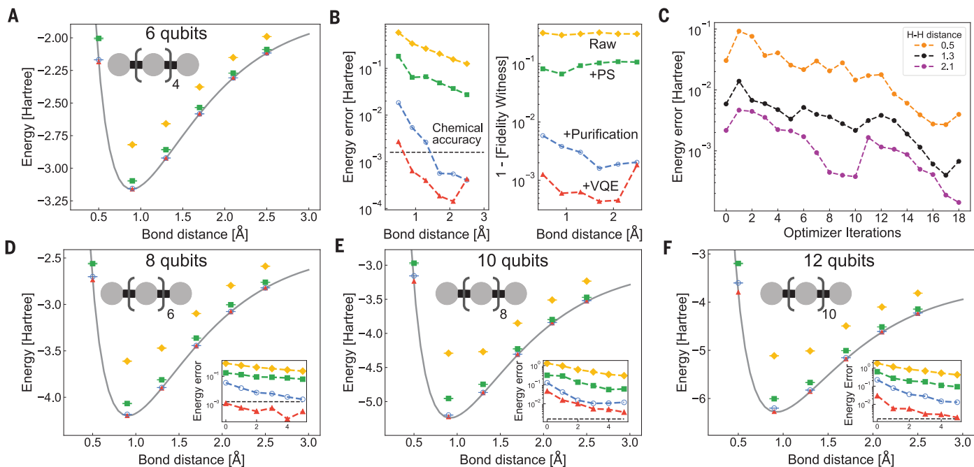
Fig. 2. Static and VQE performance on hydrogen chains. Binding curve simulations for H 6 , H 8 , H 10 , and H 12 with various forms of error mitigation. (A and D to F) Comparison of Sycamore’s raw performance (yellow diamonds) with postselection (green squares), purification (blue circles), and error-mitigated combined with variational relaxation (red triangles). For all hydrogen systems, the raw data at 0.5-Å bond length is off the top of the plot. The yellow, green, and blue points were calculated by using the optimal basis rotation angles computed from a classical simulation; thus, the variational optimization shown here is only used to correct systematic errors in the circuit realization. (B) The absolute error and infidelity for the H 6 system. For all points, we calculated a fidelity witness described
