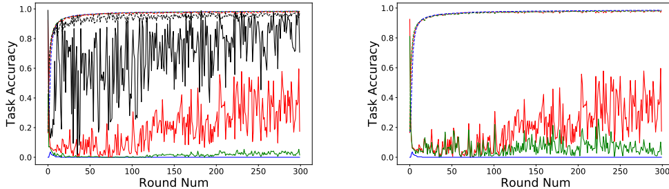
(a) Norm clipping bound: Blue - unattacked baseline, (b) Gaussian noise (norm bound = 5). Red: \sigma = 0 , Green: 3, Red: 5, Black: 10 green: \sigma = 0.025 , blue: unattacked baseline
