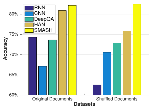
Figure 7: The classification performance of different methods with the original and shuffled documents in related article recommendation. SMASH uses the paragraph- and sentence-level hierarchies.
