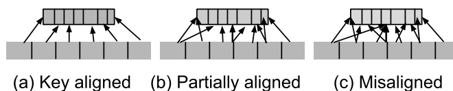
Figure 6: Classes of views based on the commonality of the view and base table key columns.
