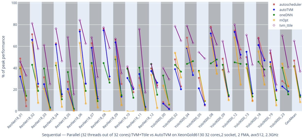
Figure 9: Comparison with AutoTVM, AutoScheduler, oneDNN, Mopt for AVX512 (Intel Xeon Gold 5220 and 6130), shown as percentage of machine peak. The left side of each line is the sequential performance and the right side is the parallel performance for the same convolution sizes. The last entry is the geometric mean for each tool, for the sequential and parallel case.
