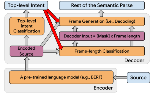
Figure 1: The proposed model architecture. By decoupling the top-level intent prediction from the output prediction, we perform conditional generation of the frame length and parse upon the top-level intent.
