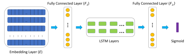
Figure 4: The Architecture of our RNN Model.
