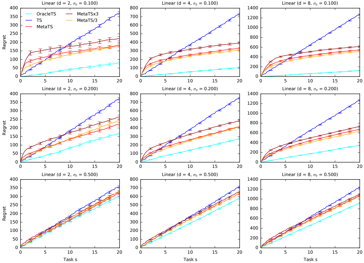
Figure 4. MetaTS in d -dimensional linear bandits with a varying dimensionality d and instance prior width \sigma_0 .
