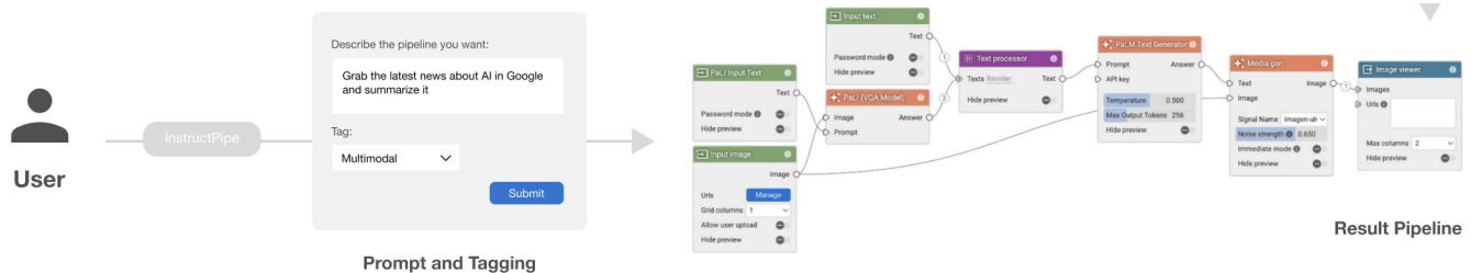
Figure 1: We demonstrate InstructPipe, an AI assistant that enables users to start prototyping machine learning (ML) pipelines with text instructions. To achieve this, InstructPipe leverages two LLM modules and a code interpreter to generate pseudocode of a target pipeline, and the interpreter renders a pipeline in the node-graph editor for further human-AI collaboration.
