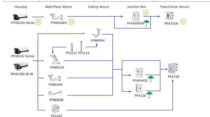
Camera Housing Wall/Plane Mount Ceiling Mount Junction Box Pole/Corner Mount
