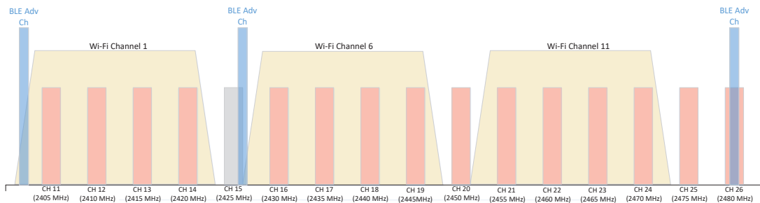
Figure 9 - All Type X Channels Shown with Standard Wi-Fi and Bluetooth Low Energy (BLE) Advertising Channels
