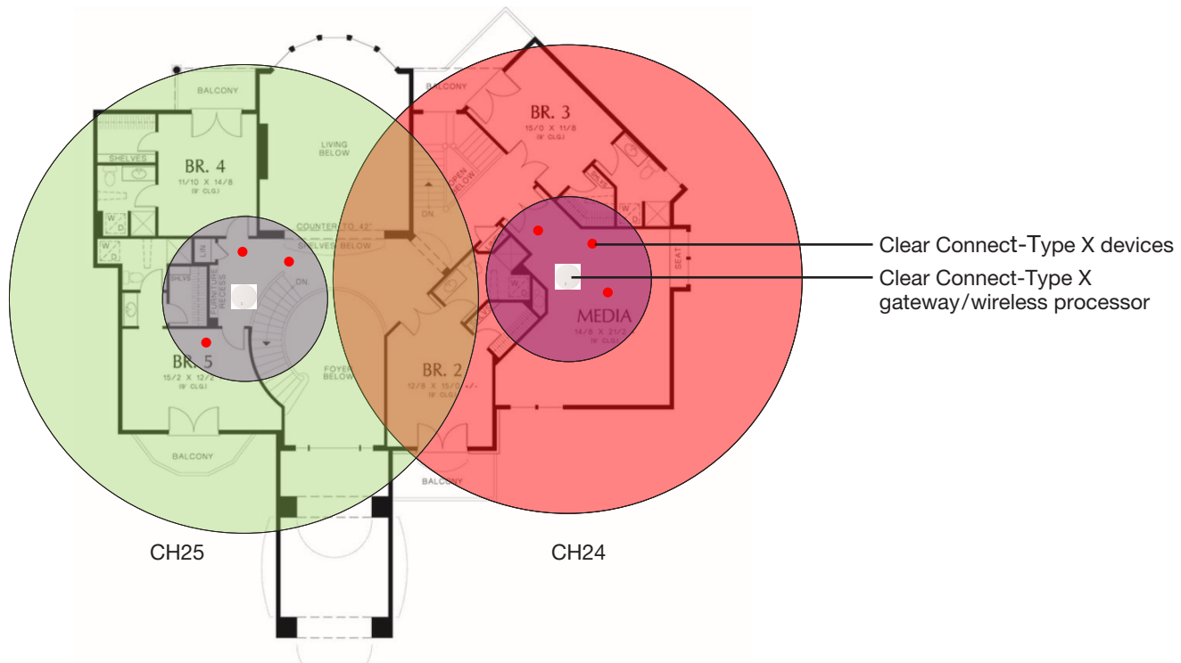
Figure 2 - Upper floor of residence with two gateways/wireless processors on the floor
