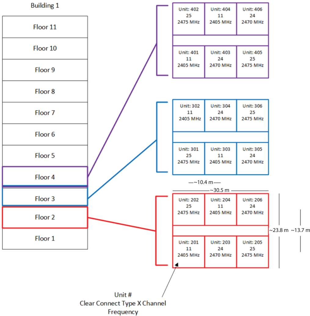
Figure 17 - Multiple Dwelling Unit with Multiple Floors and Multiple Units per Floor
