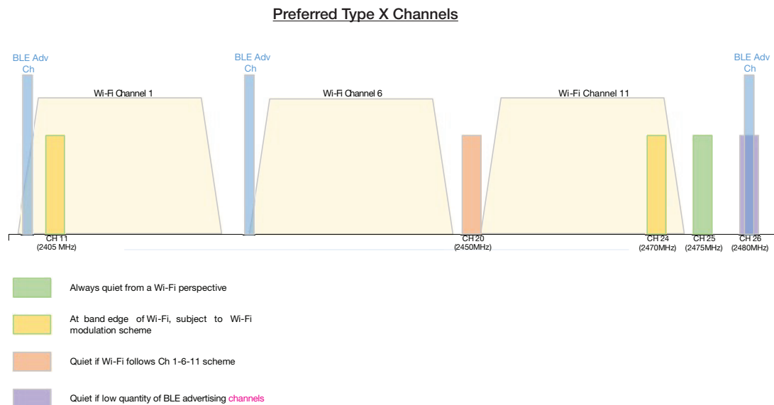
Figure 10 - Type X Preferred Channels Shown with Standard Wi-Fi and Bluetooth Low Energy Advertising Channels
