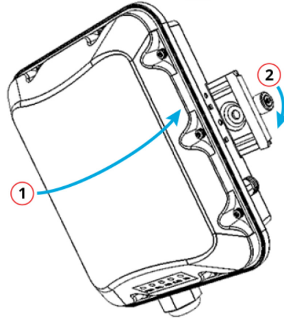
1. Snap the AP to the mounting bracket 2. Tighten the captive screw
