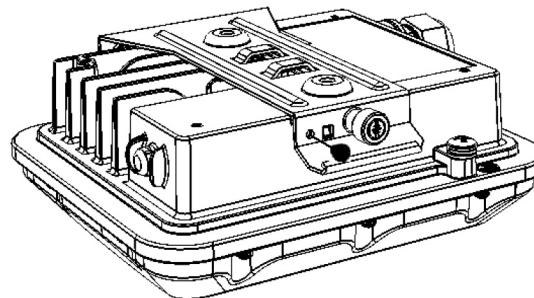
FIGURE 12 Locking the Mounting Bracket to the AP
