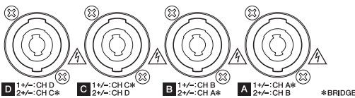
PC-D series
