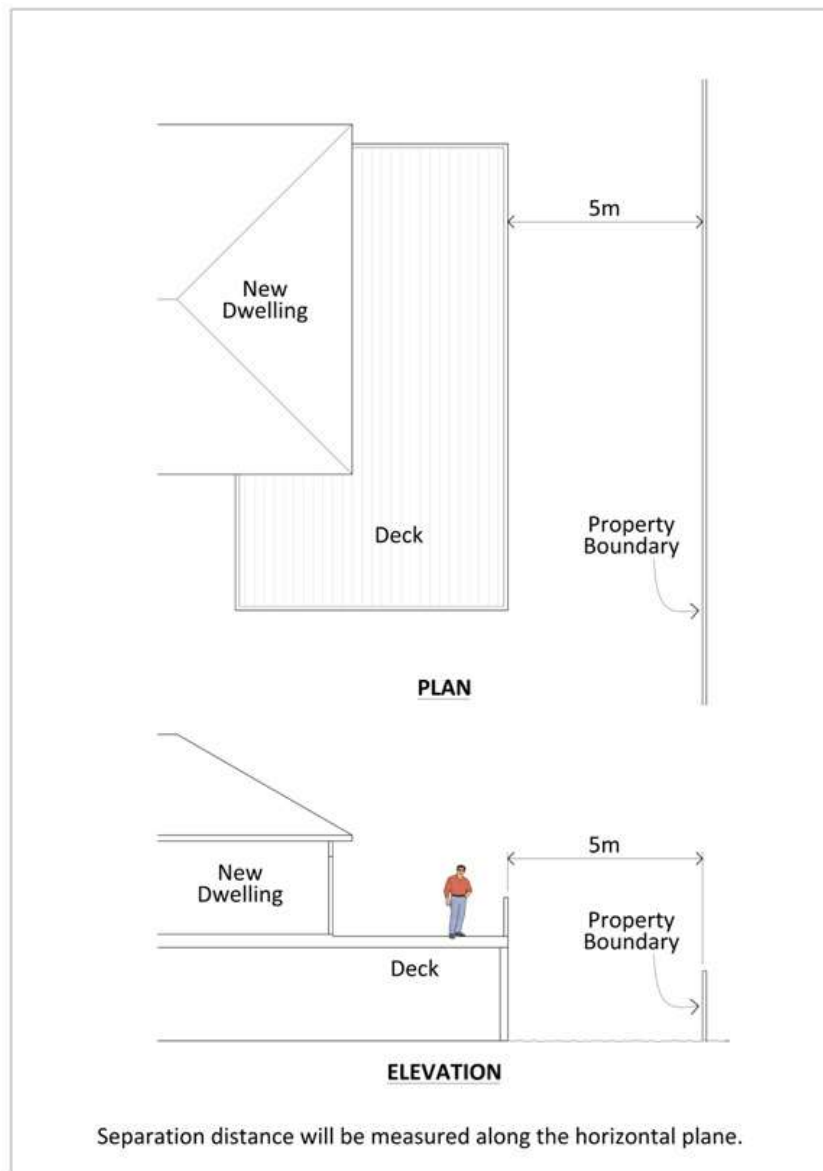
Figure 5.4.9a: Upper-floor setbacks for separation and privacy
