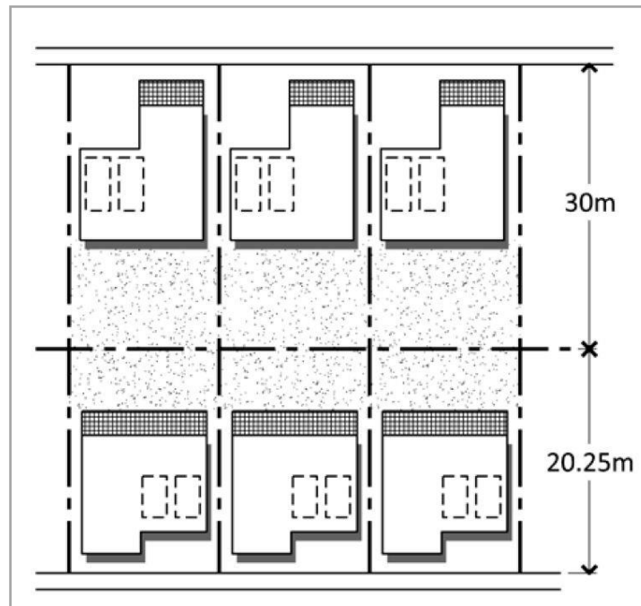
Figure 1.4.7gf: Design for deeper back yards to allow sun in south-facing parts of the site, front setbacks of at least 3m allow for a front porch or deck
