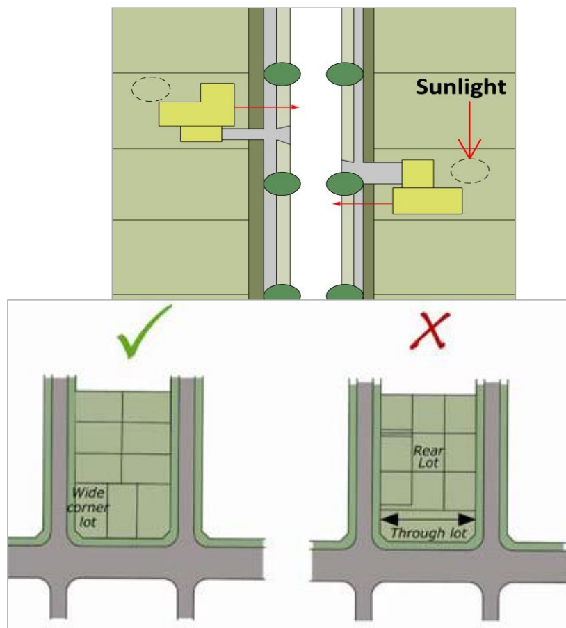
Figure 1.4.1l: Blocks and allotments have been located and designed to ensure dwellings and allotments receive a good level of sunlight
