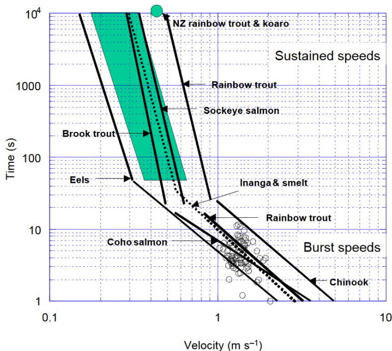
Figure 7-3 - Figure 3 from Boubée et al. (1999), Durations that NZ native and foreign fish species are able to maintain swimming velocities. The shaded area represents sustained speeds for common bully, shortfinned eels, smelt, banded kokopu and inanga with sizes between 40 and 70 mm. The circles show burst speeds for smelt and inanga with average size 70 mm.
