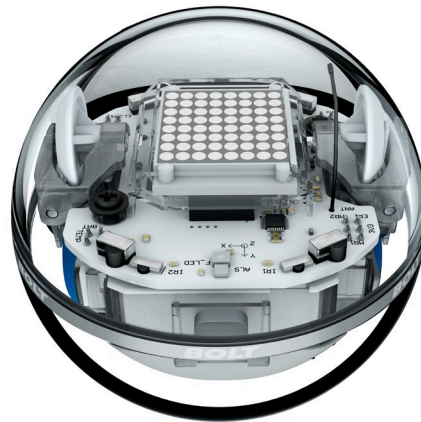
Sphero BOLT™
