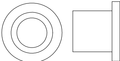
026-01M0780 .65" LONG HEAVY FLANGED SPACER
