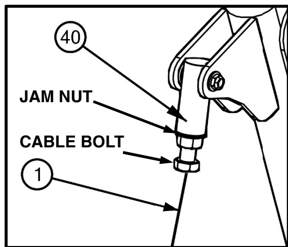
INSTALLED VIEW
