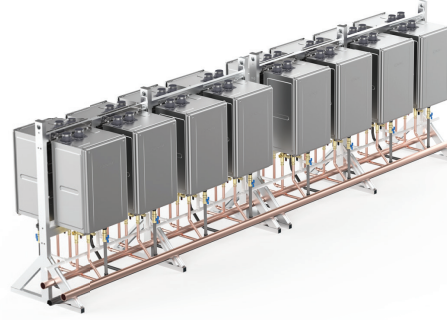
16 Units, Back to Back Floor Standing System
