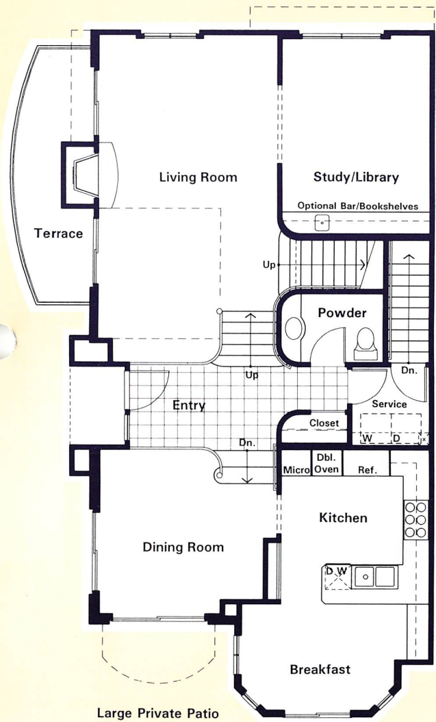
LOWER FLOOR
