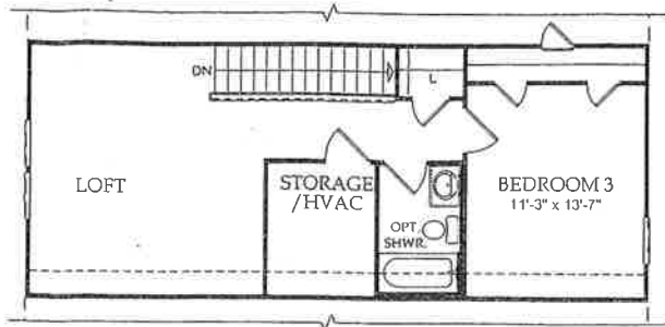
Loft Opt. @ Second Floor
