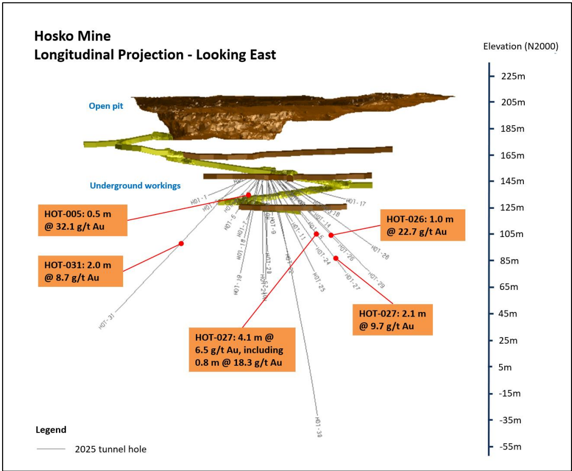
Figure 1) Longitudinal projection of the Hosko mine with the 2025 drilling program drill hole traces.
