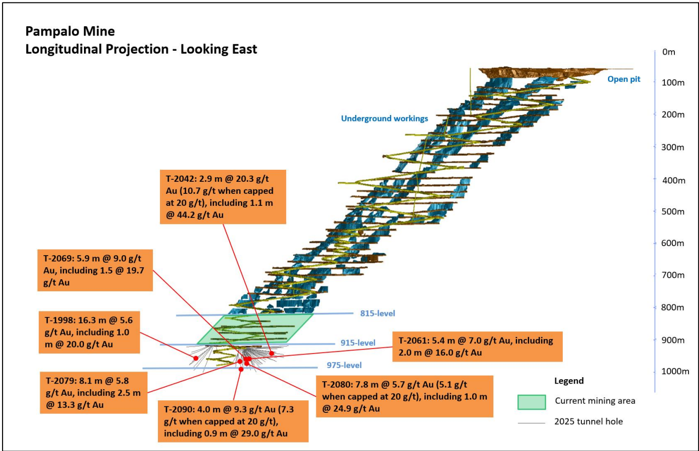
Figure 1) Longitudinal projection of the Pampalo mine with the 2025 drilling program drill hole traces.
