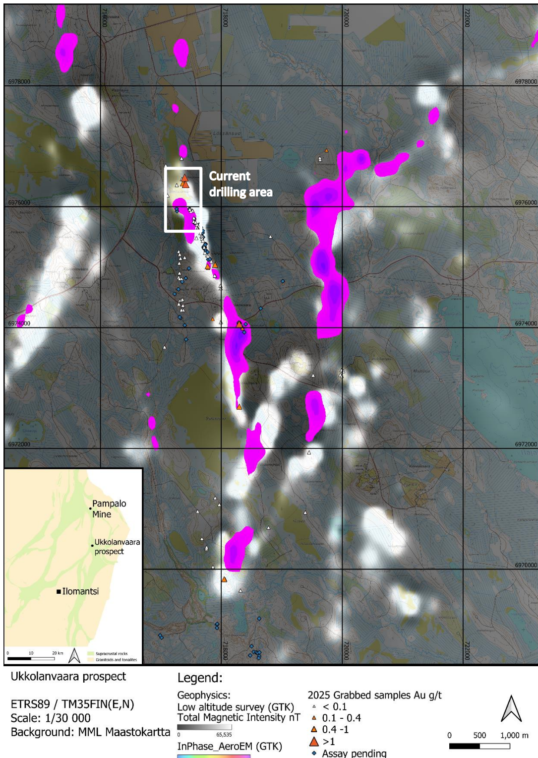
Figure 1) Outcrop samples collected in 2025 from the Ukkolanvaara prospect underlain by Total magnetic Intensity map and high ground conductivity areas illustrated by a strong In Phase response on the low altitude EM survey map.
