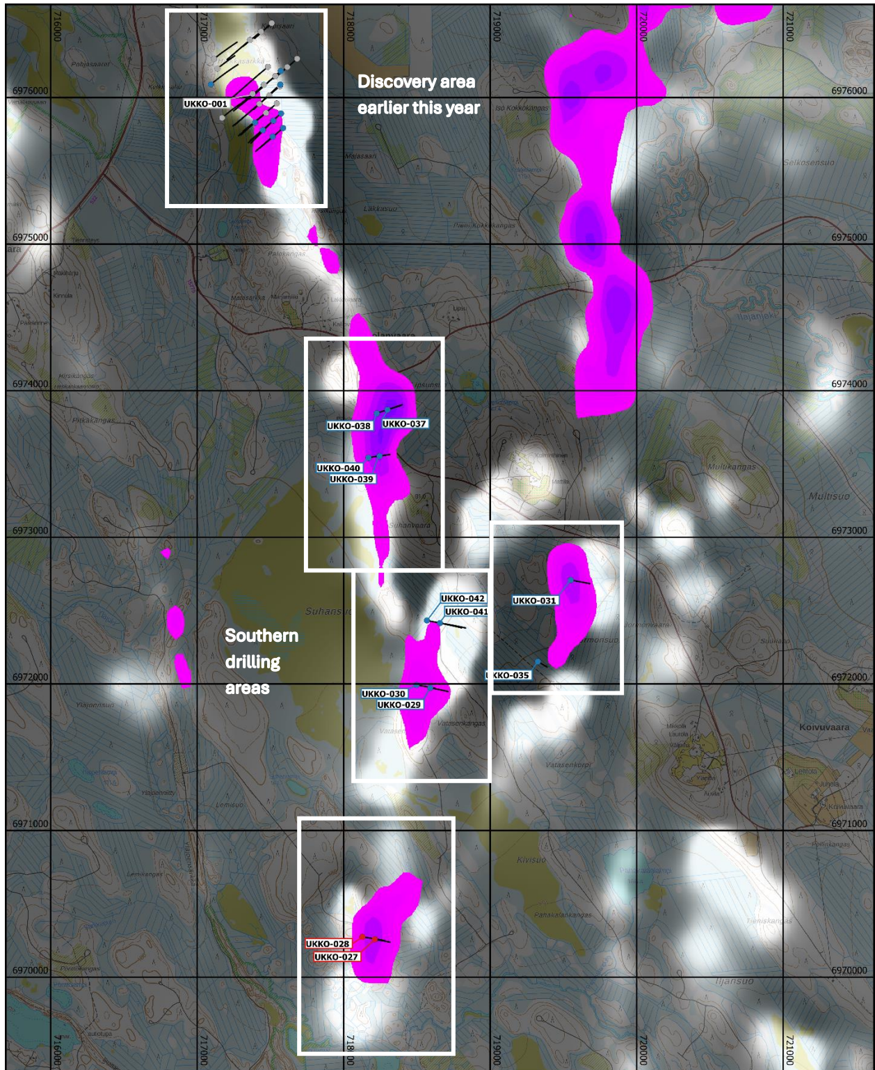
Figure 2 – Location map of the 2025 drill holes in Ukkolanvaara underlain by Total magnetic Intensity map and high ground conductivity areas illustrated by a strong In Phase response on the low altitude EM survey map.
