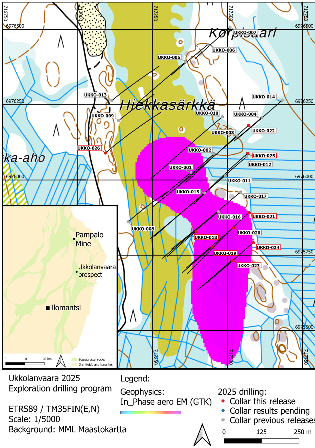
Figure 1) Location map of the 2025 exploration drilling program drillholes collars underlain by high ground conductivity areas illustrated by a strong In Phase response on the low altitude EM survey map at Ukkolanvaara, Karelian Gold Line.
