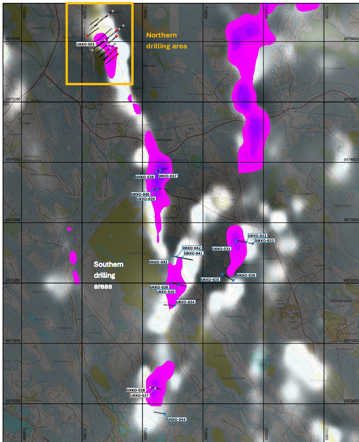
Figure 1 – Location map of the 2025 drill holes in Ukkolanvaara underlain by Total magnetic Intensity map and high ground conductivity areas illustrated by a strong In Phase response on the low altitude EM survey map.
