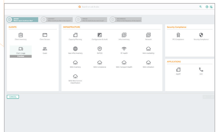
Figure 4: Reporting Wizard
