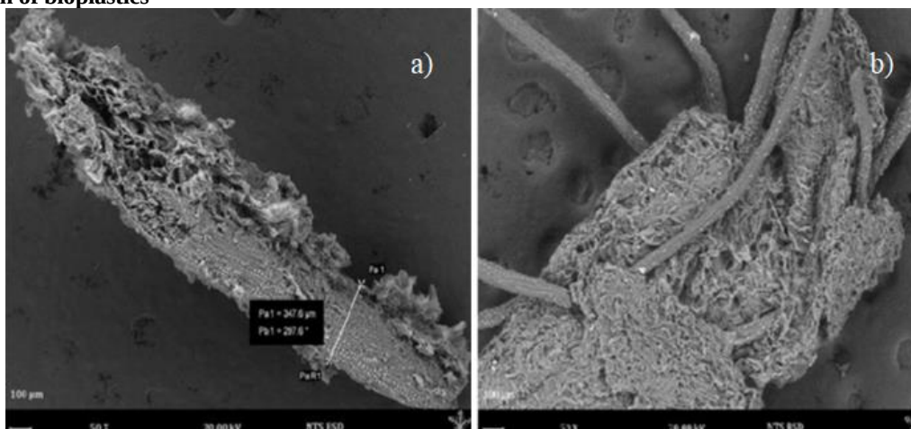
Figure 1. SEM micrographs of coconut bagasse: (a) native and (b) modified by acid hydrolysis.
