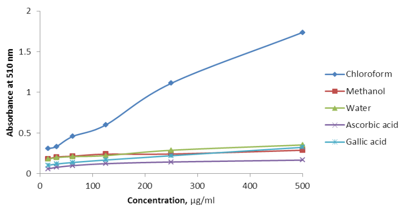
Figure 3: Reduction of ferric ions of different extracts of Tagetes erecta stems by ortho -phenanthroline colour method.
