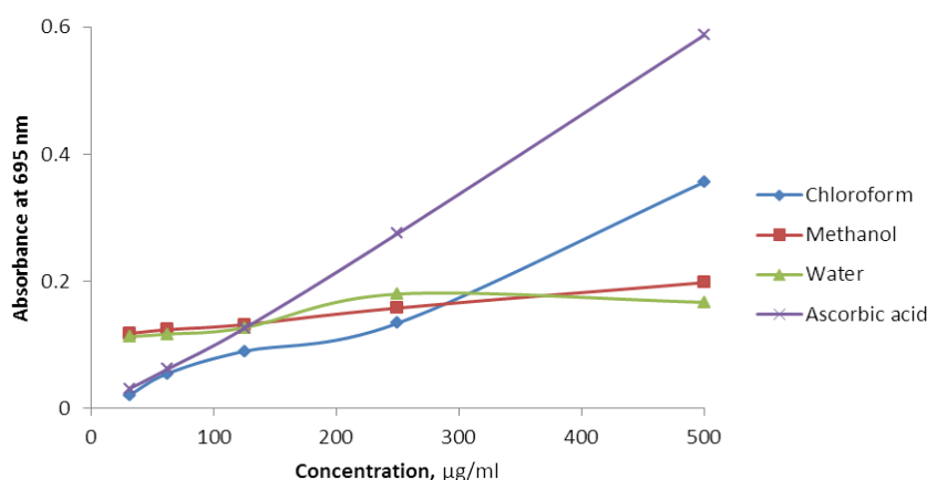
Figure 2: Total antioxidant capacity of different extracts of Tagetes erecta stems with standard.
