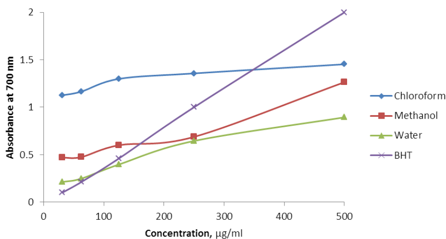
Figure 1: Reducing power assay of different extracts of Tagetes erecta with standard.
