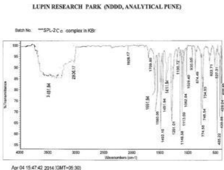
Figure-4: IR Spectrum of Co(NOMBAP) 2 ·H 2 O complex.
