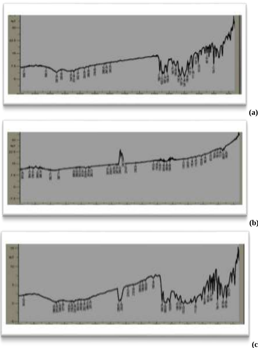
Fig 1.FTIR study
