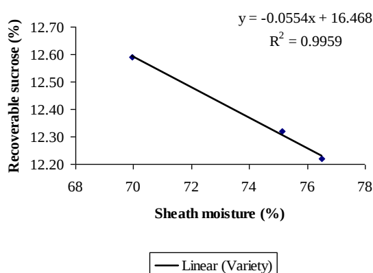
Figure 1. Linear regression between sheath moisture and recoverable sucrose among three sugarcane varieties grown at Metahara Sugar Estate.
