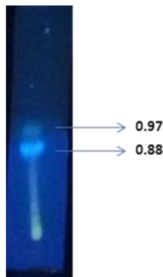
Figure 2: Compounds separated by Thin Layer Chromatography.
