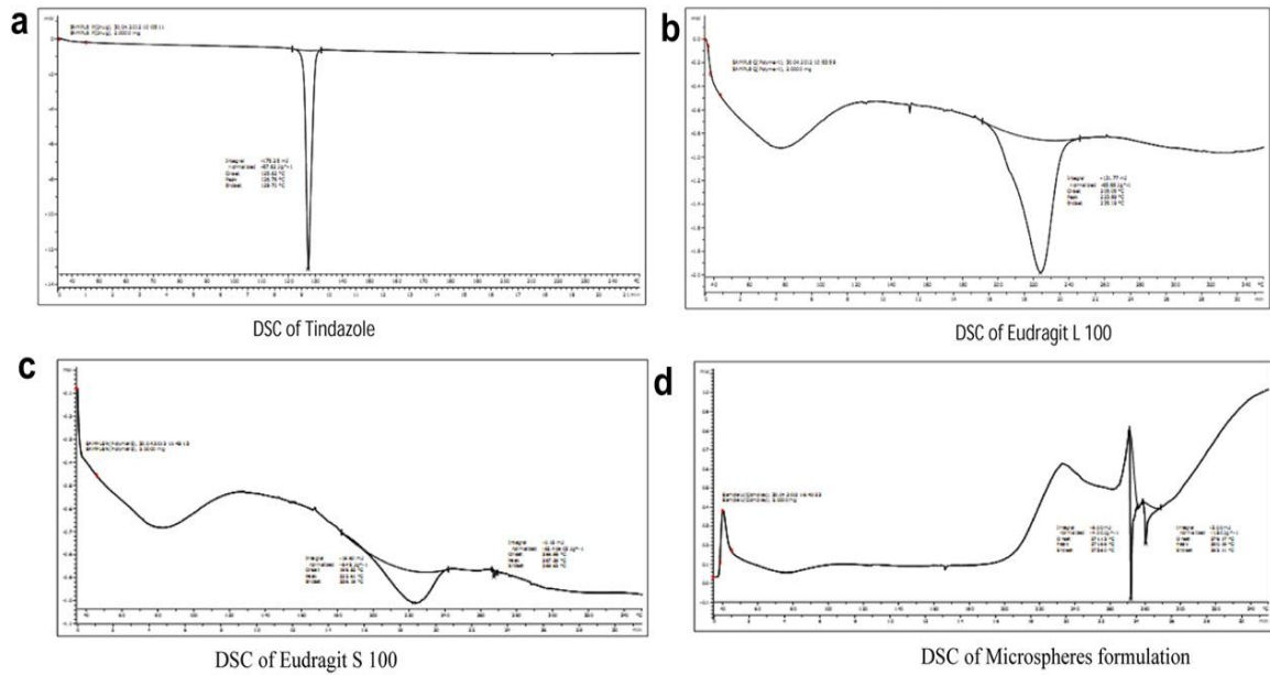
Figure 5: DSC RESULTS.
