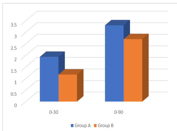
Graph 03: Comparison of mean score of NSS in between groups.
