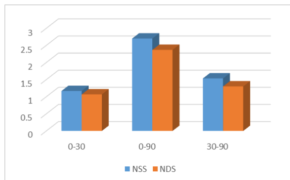
Graph 02: Mean difference of Group B.
