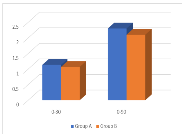
Graph 04: Comparison of mean score of NDS in between groups.
