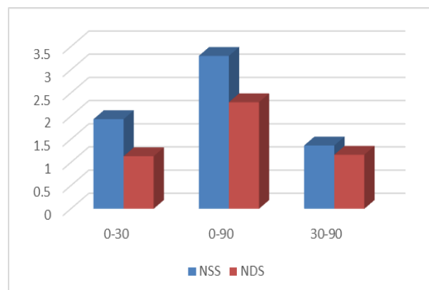
Graph 01: Mean difference of Group A.
