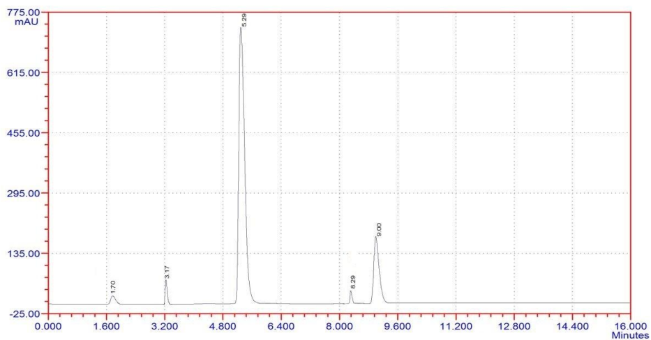
Figure 8: Peroxide degradation chromatogram of PNS and FTP.
