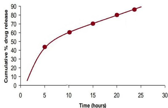
Graph 3: In- Vitro Drug Release from Microsphere optimized formulation (F6).
