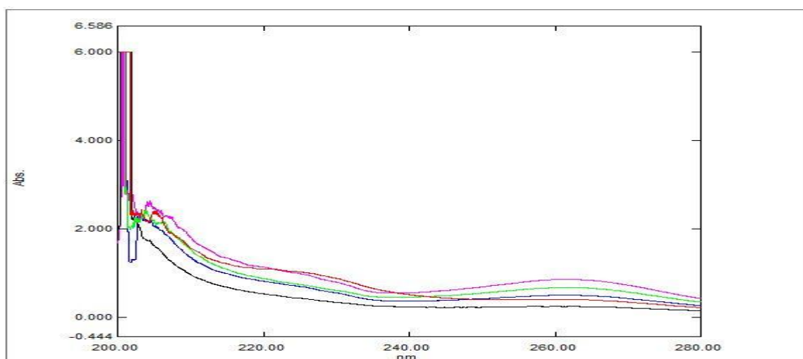
Graph.1: UV spectra of Mometasone at distinctive concentrations.
