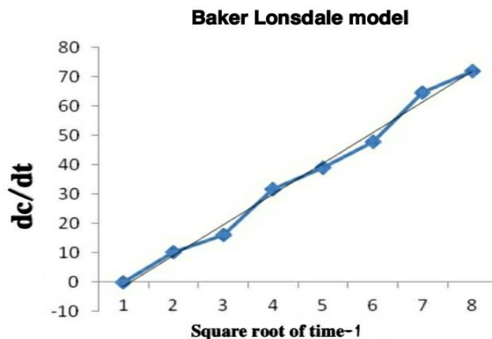
Graph.5: Baker Lonsdale model of drug release Kinetics (F6).
