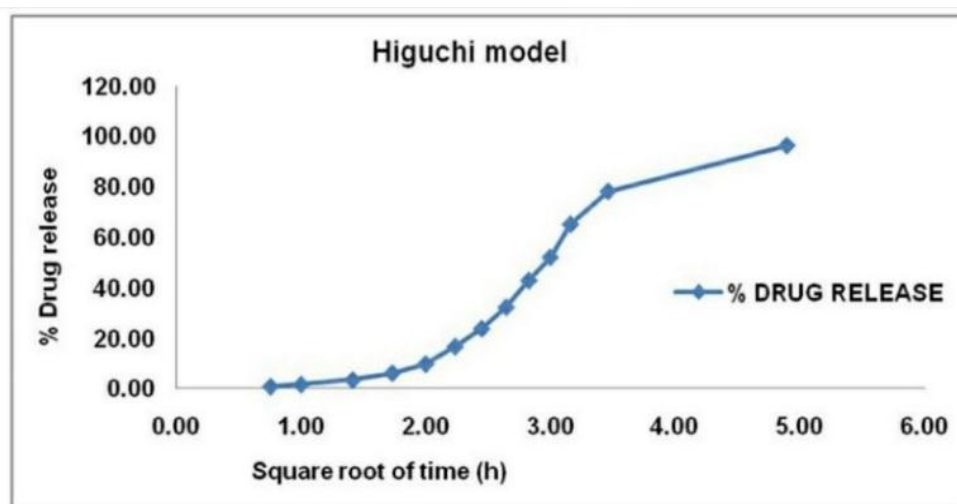
Graph 4: Higuchi model of drug release Kinetics (F6).
