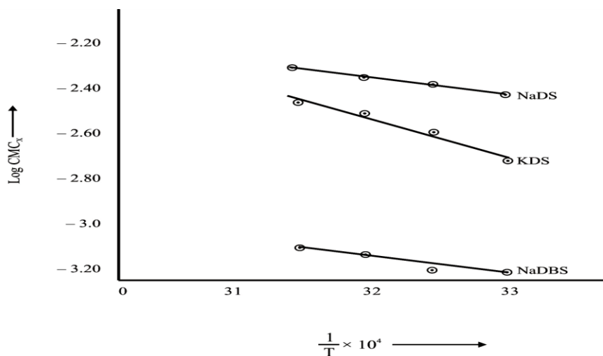
Figure 2: Plots of \log \text{CMC}_x VS \frac{1}{T} of surfactants in presence of 0.5 M Urea in 2.5% Butanol-water system at different temperatures.
