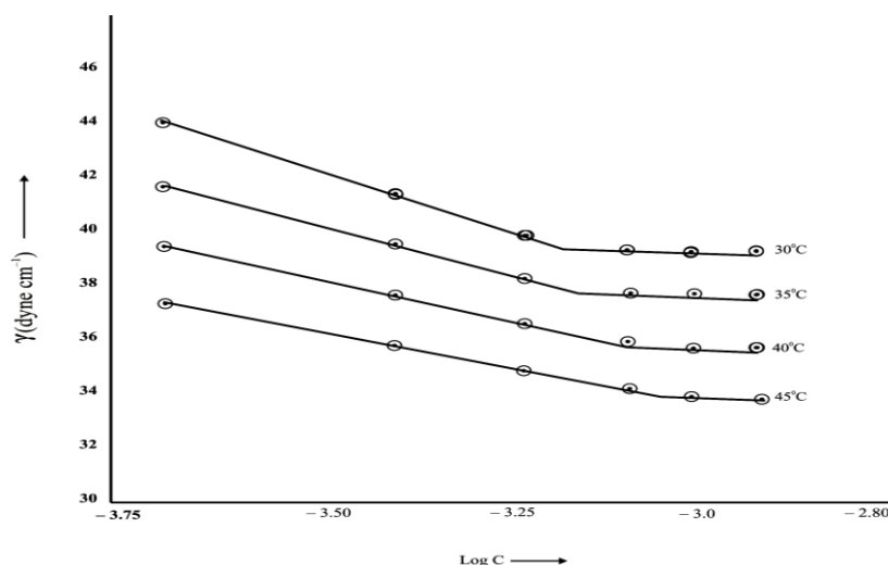
Figure 1: Plots of surface Tension VS Log C of Nadbs in presence of 0.5 M Urea in 2.5% Butanol-water system at different temperatures.
