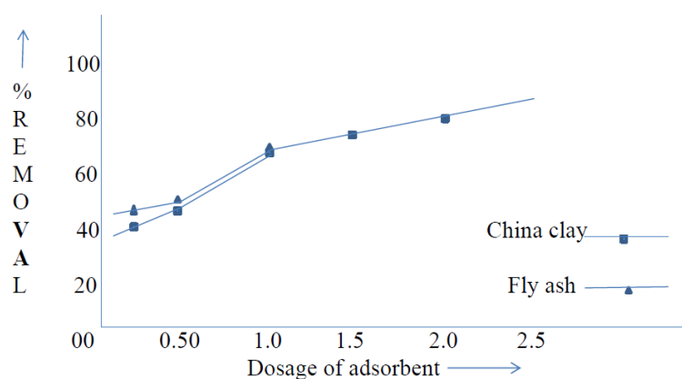
Figure 4: Effect of adsorbent dosage vs Pb(II) concentration at 180 min of contact time, pH 4.5 and 1.0 gm adsorbents.
