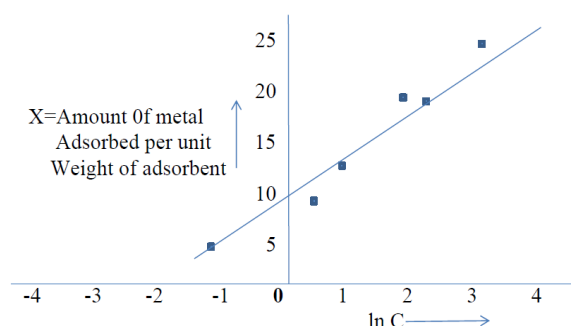
Figure 6: Temkin adsorption isotherm of lead on Fly ash.
