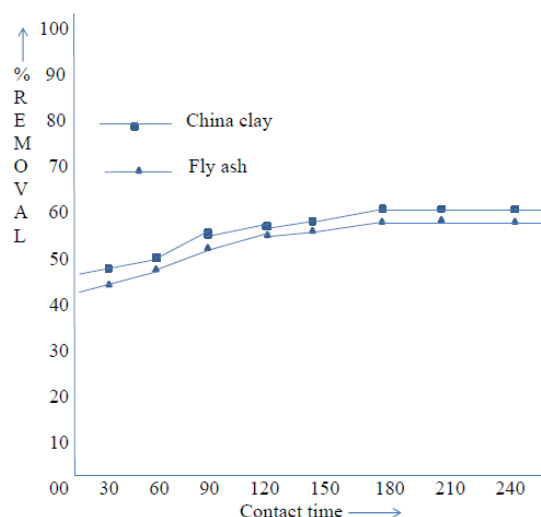
Figure1: Percentage removal of Pb(II) (25ppm) on adsorbents.
