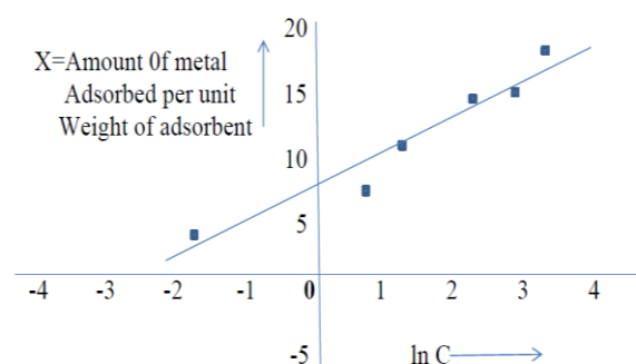
Figure 5: Temkin adsorption isotherm of lead on China clay.
