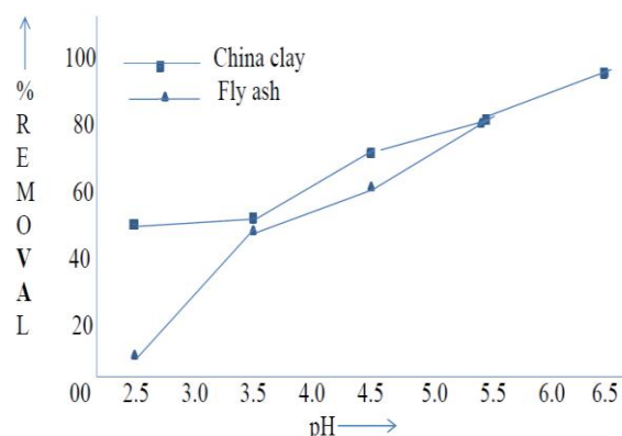
Figure 3: Effect of pH on lead removal (25 ppm solution) through adsorption on adsorbents.
