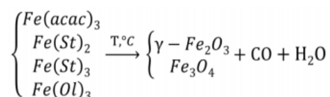
Fig. 2: Reaction resulting in the fromation of nanoparticles via given precursors.
