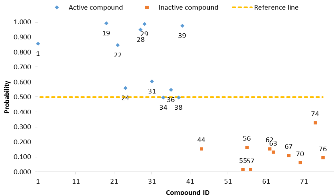
Figure 2: Graphical representation of the prediction made on test set compounds.
