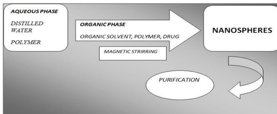
Figure 3: Solvent displacement.
