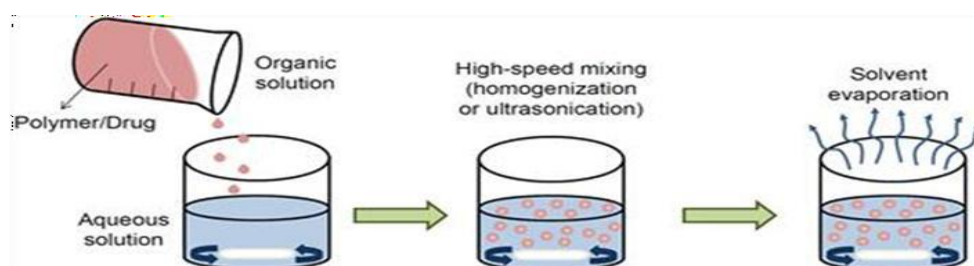
Fig. 1: Solvent evaporation.
