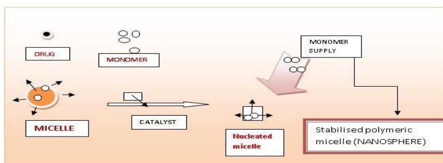
Figure 2: Polymerisation.
