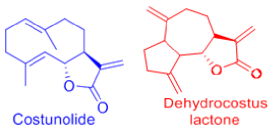
Figure 2: Structure of CE(C 15 H 20 O 2 ) and DE(C 15 H 18 O 2 ).
