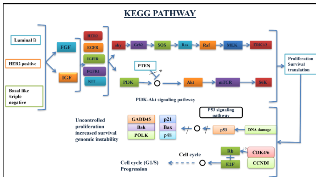
Figure 3: Schematic sketch for KEGG pathway for breast cancer.
