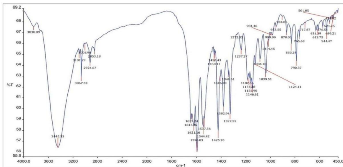
Fig. 2: FTIR spectra of Metformin Hydrochloride.
