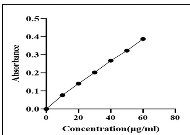
Fig. 3: Calibration Curve of Metformin Hydrochloride in Distilled Water.
