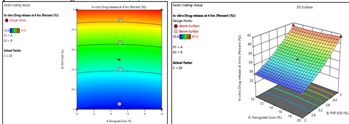
Fig. 6: The 2D contour plot and 3D response surface illustrates the combined effect of fenugreek gum and PVP K30 concentrations on In-vitro drug release at 4 hrs in sustained release tablets.
