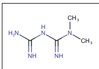
Fig. 1: Chemical structure of Metformin Hydrochloride.
